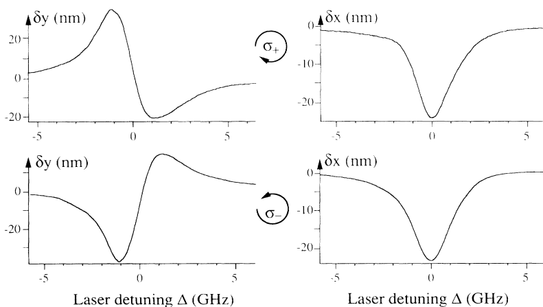
FIG. 3. Experimentally measured beam displacement. Shown is the amplitude of the signal at the Larmor frequency, out of phase with respect to the intensity modulation perpendicular (left) and parallel (right) to the magnetic field as a function of the laser frequency. The upper row was measured with a right circularly polarized probe beam; the lower row, with a left circular polarization.
