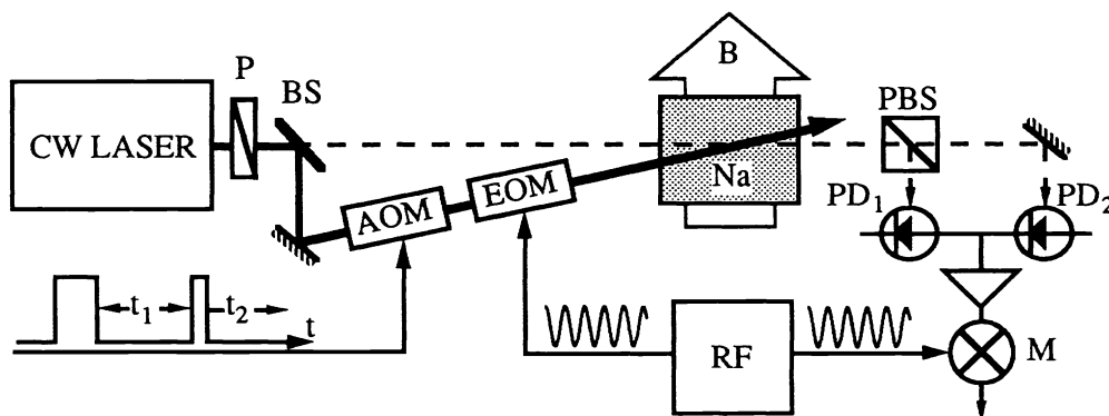
Figure 2: Experimental setup used for the investigation of atomic multilevel systems. P = polarizer, BS = beam splitter, AOM = acoustooptic modulator, EOM = electrooptic modulator, RF = radio-frequency synthesizer, B = magnetic field, PBS = polarizing beamsplitter, PD 1,2 = photodiodes, M = mixer.
