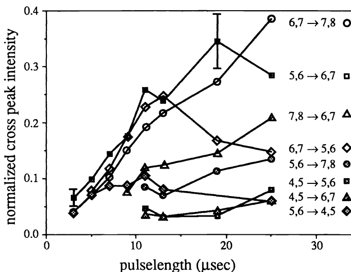
Figure 7: Normalised intensity of cross peaks in two dimensional sublevel spectra of the Na ground state as a function of the length of the second pulse.
