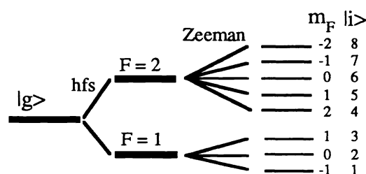
Figure 1: Level structure of the Na ground state.
