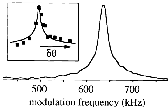
Figure 9: Example of a magnetic resonance spectrum of the Na ground state recorded with the setup of figure 8. The inset shows the dependence of the signal amplitude on the angle of incidence of the probe beam in a region close to the critical angle.
