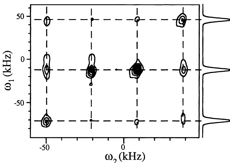
Figure 6: Example of a two dimensional spectrum demonstrating the possibility to use this method for observing 'forbidden' Raman transitions. The vertical axis represents the double quantum ( |\Delta m_F| = 2 ) spectrum, while the horizontal axis corresponds to the single quantum spectrum.
