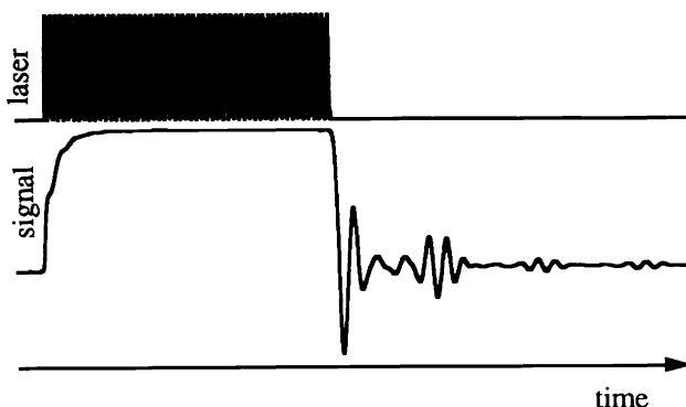
Figure 3: Response of the Na atoms to a pulse of polarization-modulated polarized light after phase sensitive detection at the modulation frequency.
