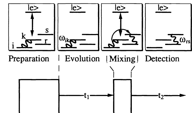
Figure 5: Schematic representation of the two-pulse sequence used for twodimensional spectroscopy and the effect on the atomic system. The individual periods are labelled with their conventional names.
