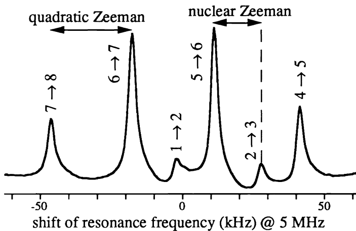
Figure 4: Fourier transform of the free induction decay signal shown in figure 3.
