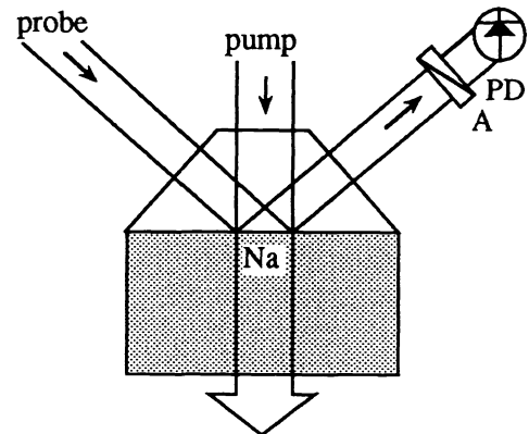
Figure 8: Principle of evanescent-wave spectroscopy of atomic multilevel systems.
