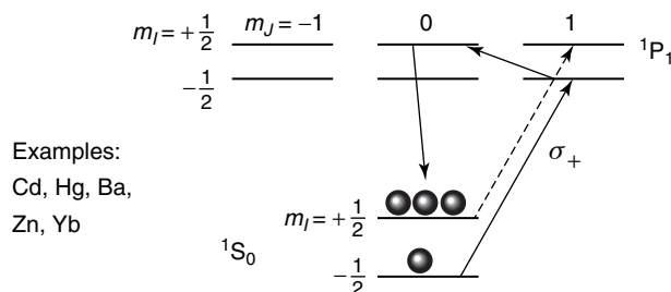
Figure 8 Polarization of nuclear spin reservoirs in diamagnetic ground states
