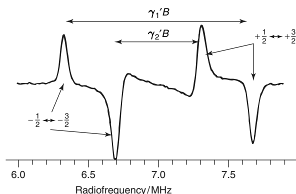
Figure 15 Raman heterodyne spectrum of \text{Pr}^{3+}:\text{YAlO}_3 in a weak magnetic field
