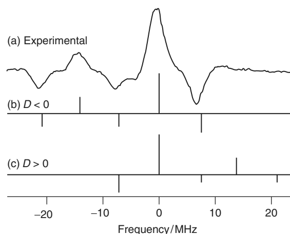
Figure 13 Comparison of the experimental spectrum (top) with theoretical stick spectra for negative and positive quadrupole coupling
