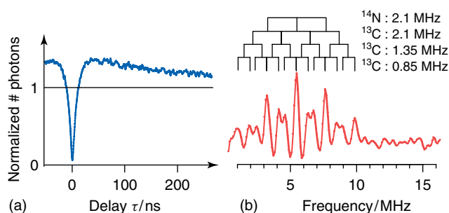
Figure 6 (a) The strong anticorrelation for delay \tau = 0 proves that a single N/V center is being probed. (b) The ESR spectrum of a single N/V center, with resolved hyperfine splittings due to the nitrogen and three ^{13}\text{C} nuclear spins
