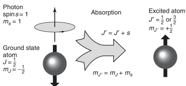
Figure 1 Conservation of angular momentum during absorption of a photon
