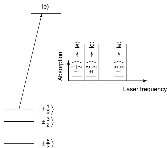
Figure 12 Principle of the measurement of nuclear quadrupole interaction by laser spectroscopy
