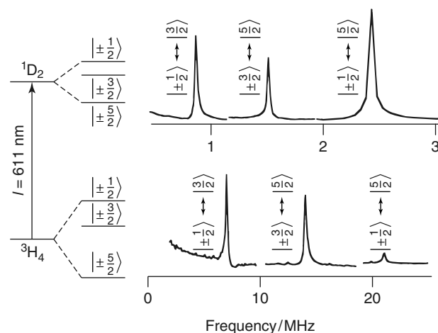
Figure 14 Example of NQR spectra obtained by purely optical excitation and detection of nuclear spin coherence. Both spectra were combined from three partial spectra which were recorded with different modulation frequencies in order to reduce distortion due to finite excitation range
