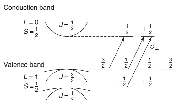
Figure 16 Optical pumping in semiconductors: level scheme for a III–V compound with tetrahedral symmetry
