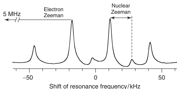
Figure 9 Example of an optically detected magnetic resonance spectrum in a strongly coupled system
