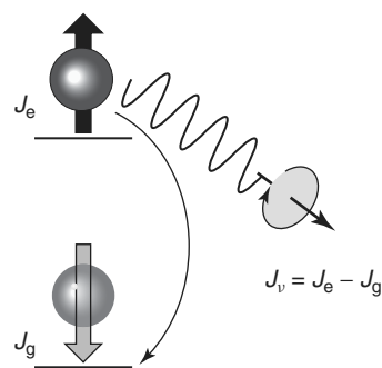
Figure 4 The polarization of the fluorescence depends on the spin state of the excited atoms
