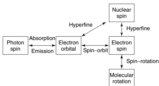
Figure 7 Summary of the most important reservoirs of angular momentum
