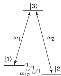
Figure 11 Raman processes couple two electromagnetic fields ( \omega_1 , \omega_2 ) with a material excitation
