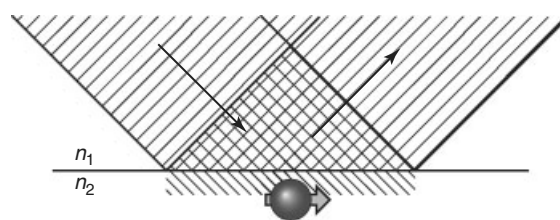
Figure 18 Principle of optical detection of magnetic resonance close to a surface. The refractive indices on both sides of the interface are denoted as n_1 and n_2
