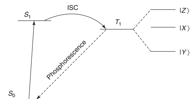
Figure 19 Principle of optically detected magnetic resonance in excited triplet states
