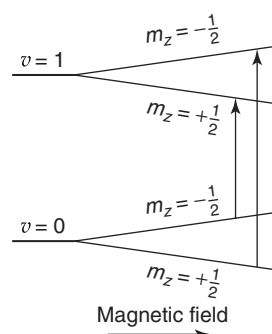
Figure 10 Principle of laser magnetic resonance
