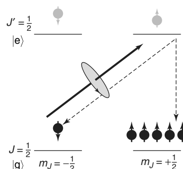
Figure 2 Principle of optical pumping illustrated for a simple atomic system
