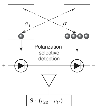
Figure 3 Principle of observation of spin polarization by transmission of optical radiation
