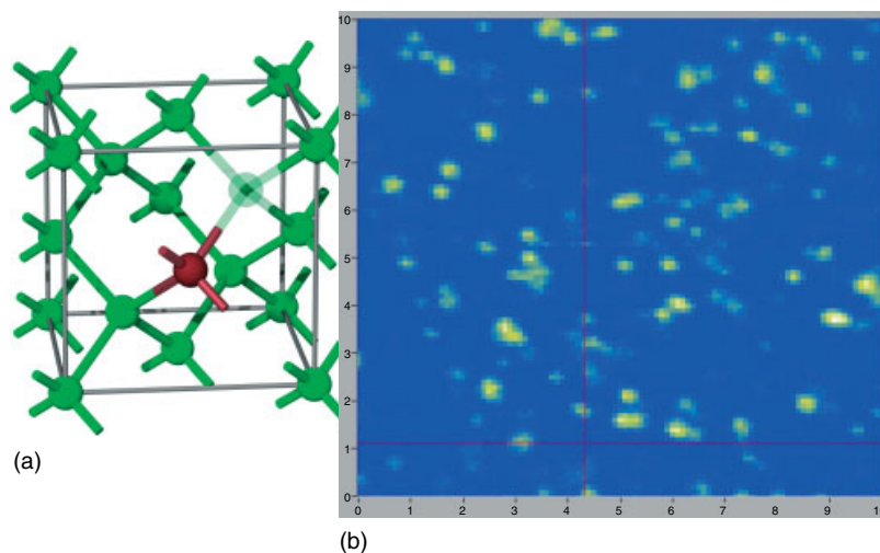
Figure 5 (a) The structure of the nitrogen-vacancy center in diamond: the red ball represents a N atom substituting for a carbon, the empty ball an adjacent missing carbon. (b) A confocal scan of a diamond crystal; each bright spot is a single N/V center
